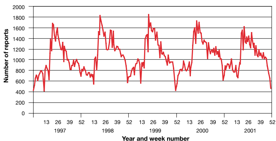
Figure 3.3: Weekly laboratory reports of Campylobacter spp. in England & Wales 1997-2001
