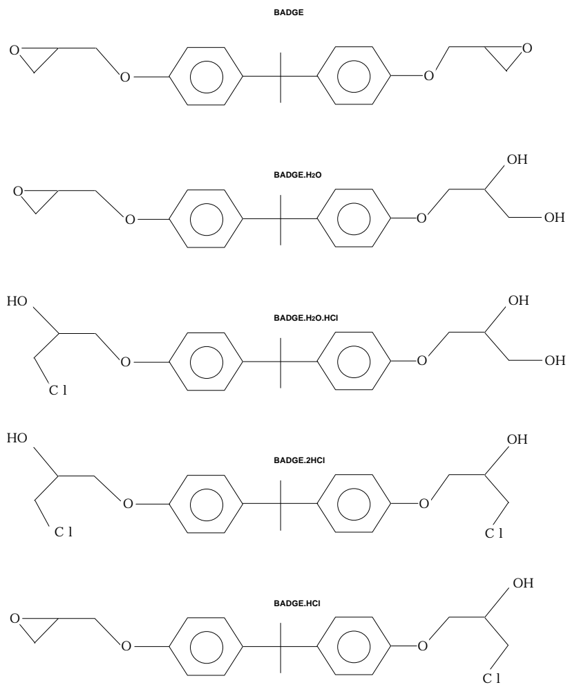
Figure 1: Structures of BADGE, BFDGE and related substances.
