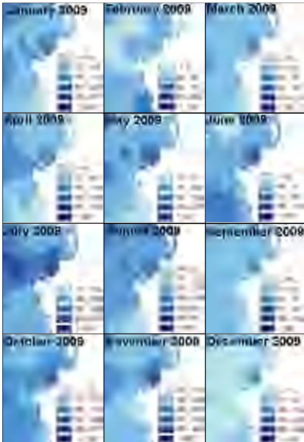
Figure 3.15: Average monthly rainfall (mm) data for 2009 (Source: Met Eireann, 2010a).
