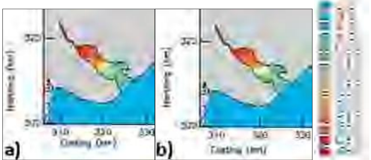
Figure 7.5: Tidal stream and residence time data for Carlingford Lough.
