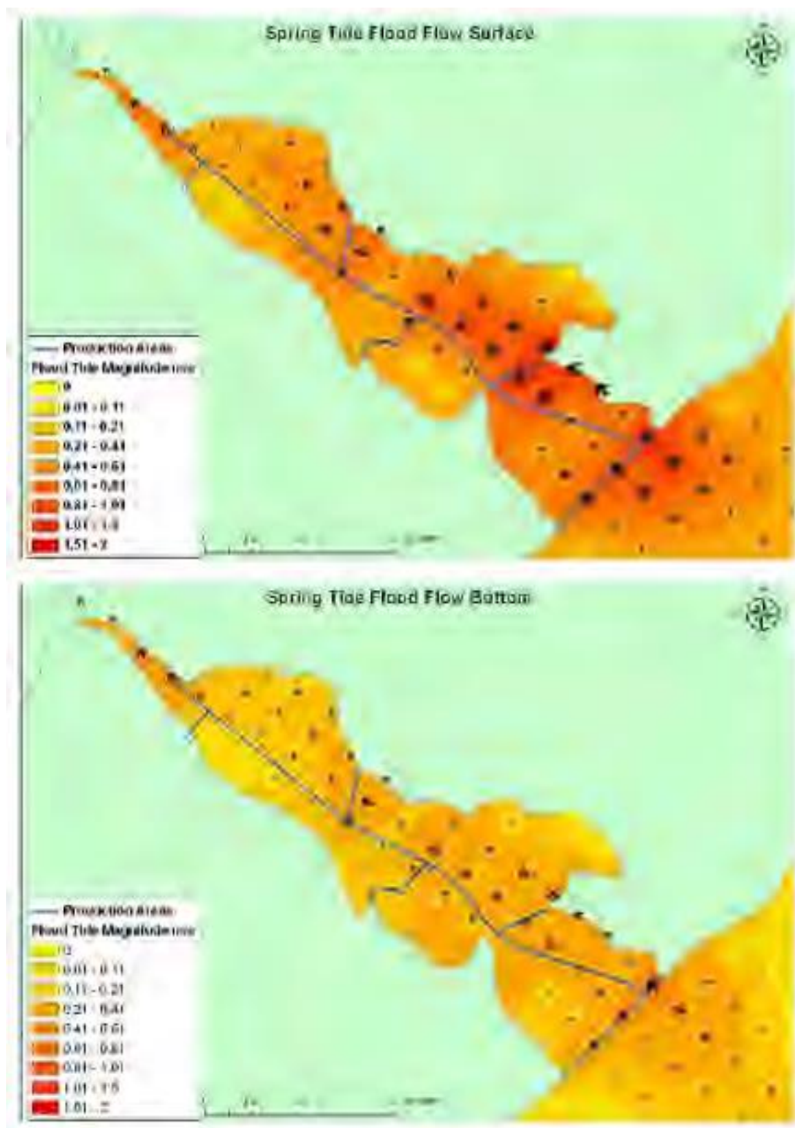
Figure 7.11: Surface and bottom current velocities and direction during a spring tide, flood flow (Source: AFBI SMILE Defit3D-Flow Model Data).
