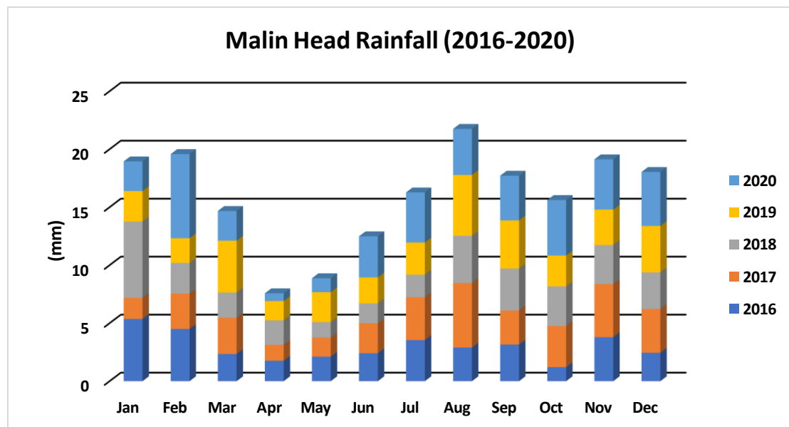
Figure 3.24: Average monthly rainfall (mm) data at Malin Head, Co. Donegal from 2016 to 2020 (Source: Met Eireann, 2021).
