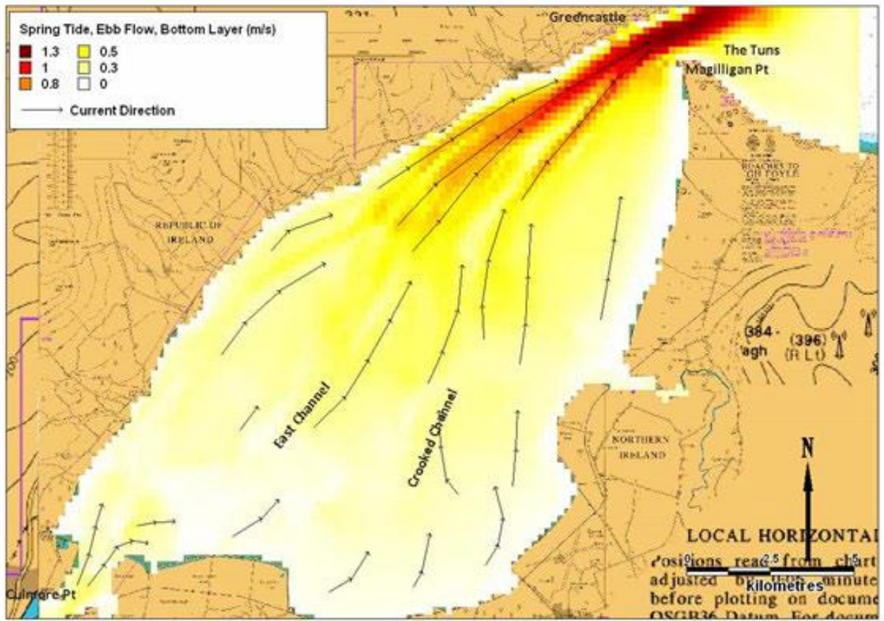
Figure 3.10: Bottom current velocities and direction during a spring tide, ebb flow at 21:30:00 November 13 th 2008 (Source: Deltares Delft3D-FLOW).
