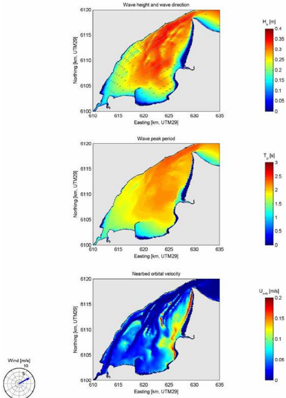
Figure 3.26: Computed wave height, peak period and near-bed orbital velocity for wind speed of 7 m/s and a wind direction of 240° (Source: Deltares, 2009).
