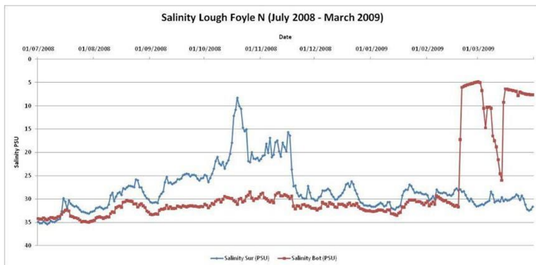
Figure 3.35: Salinity profile at Lough Foyle North EMS from July 2008 to March 2009 (Source: Loughs Agency).
