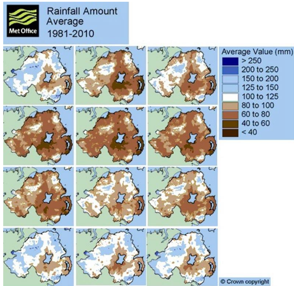
Figure 3.18: Average monthly rainfall (mm) data from 1981 to 2010 for Northern Ireland (Source: Met Office, 2010)
