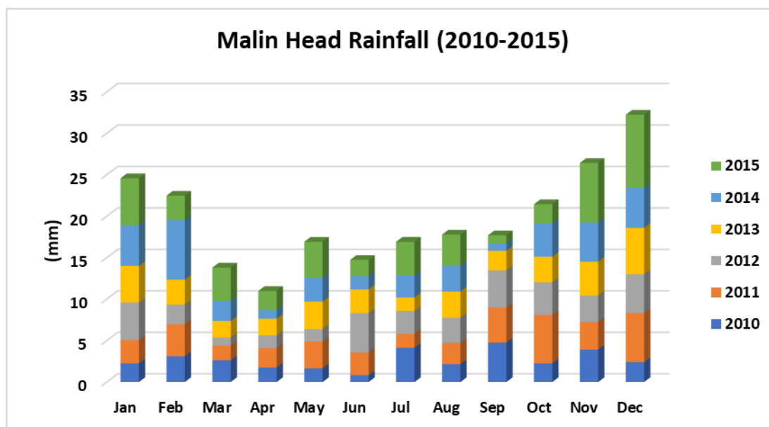
Figure 3.23: Average monthly rainfall (mm) data at Malin Head, Co. Donegal from 2010 to 2015 (Source: Met Eireann, 2021).
