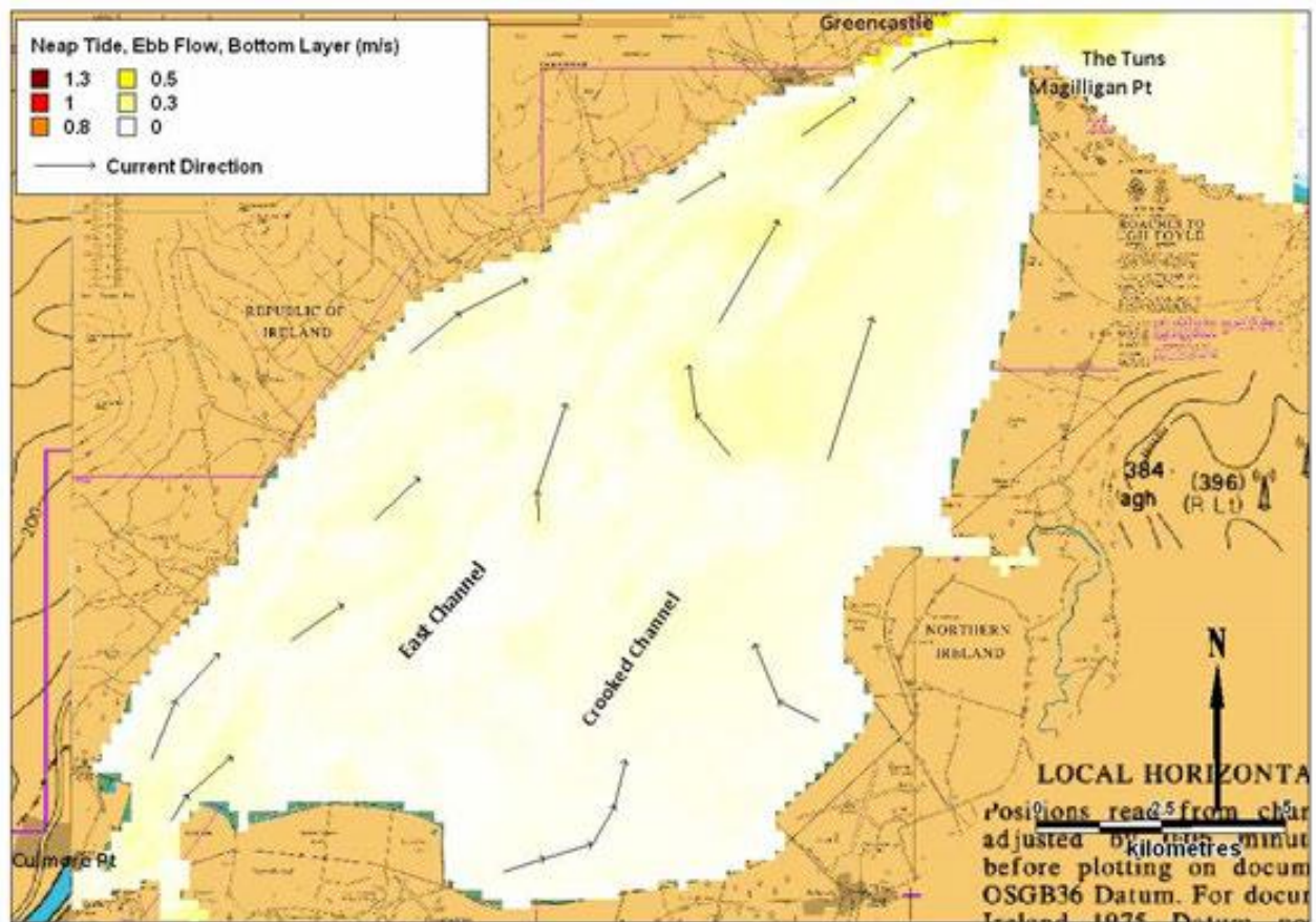
Figure 3.14: Bottom current velocities and direction during a neap tide, ebb flow at 15:30:00 November 5 th 2008 (Source: Deltares Delft3D-FLOW).
