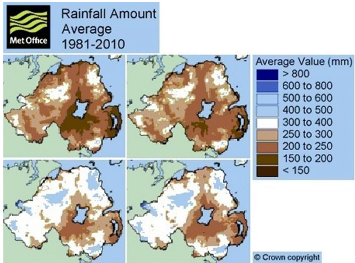
Figure 3.17: Average seasonal rainfall (mm) data from 1981 to 2010 for Northern Ireland (Source: Met Office, 2010).
