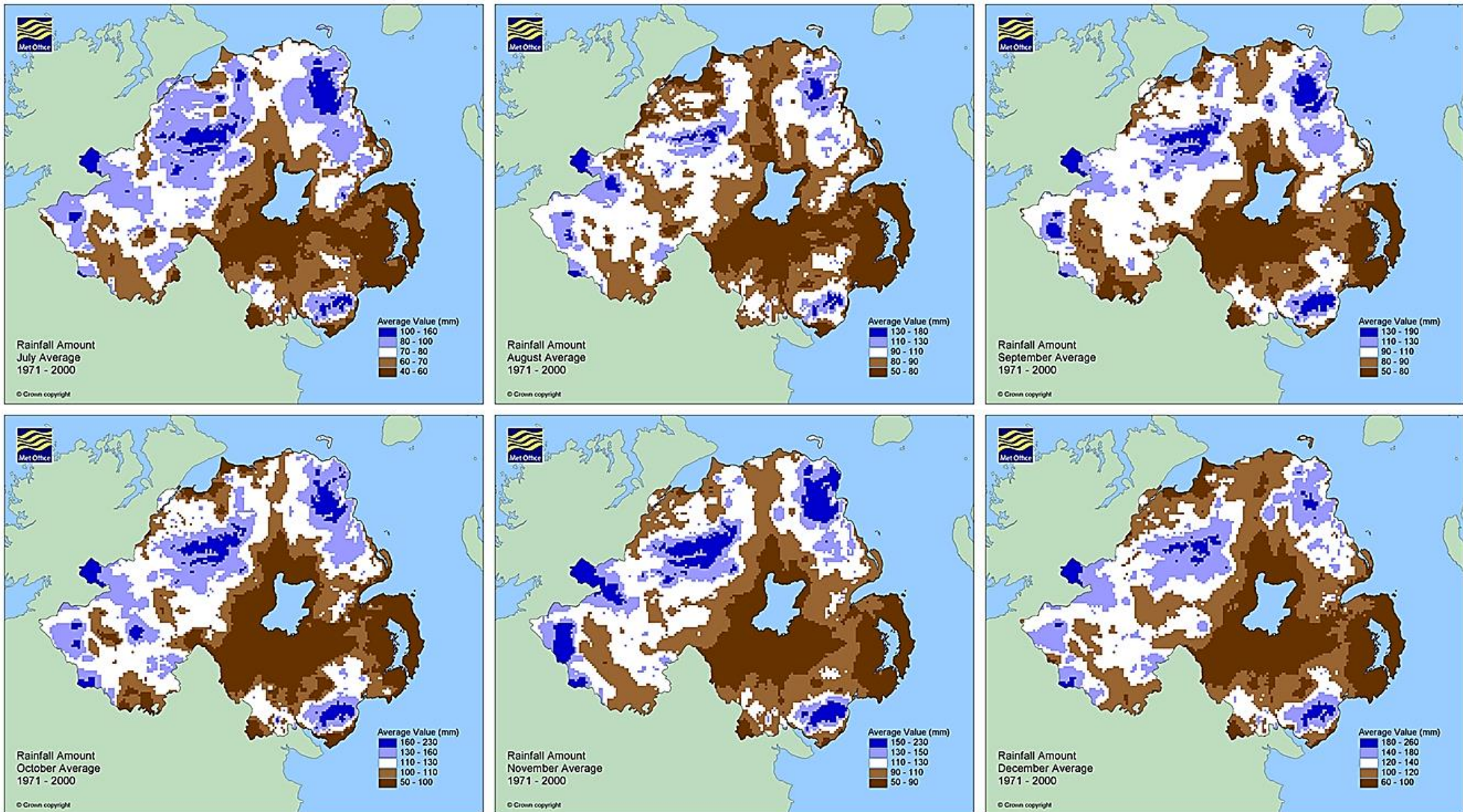
Figure 3.16: Average monthly rainfall (mm) data for July to December from 1971 to 2000 for Northern Ireland (Source: Met Office, 2010).
