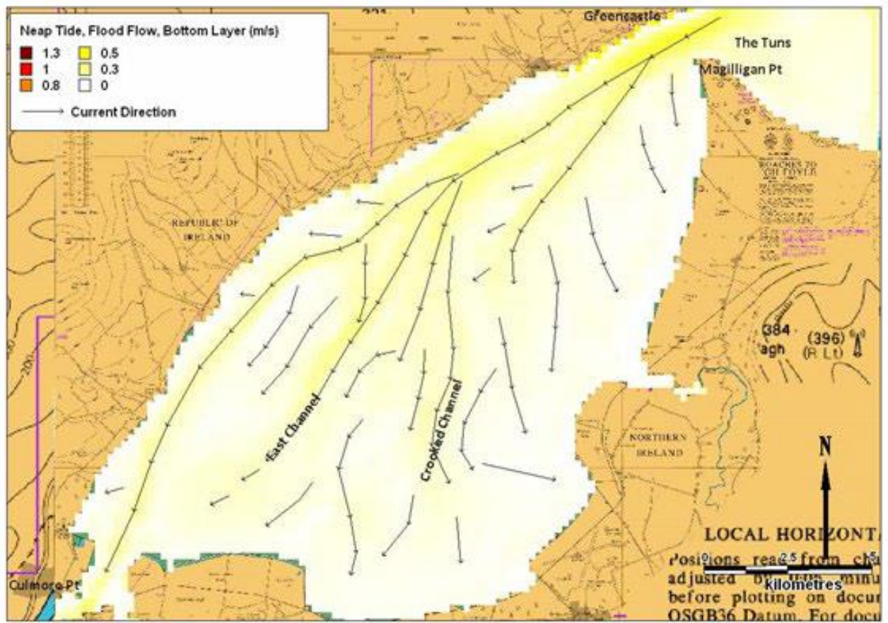
Figure 3.12: Bottom current velocities and direction during a neap tide, flood flow at 10:30:00 November 5 th 2008 (Source: Deltares Delft3D-FLOW).
