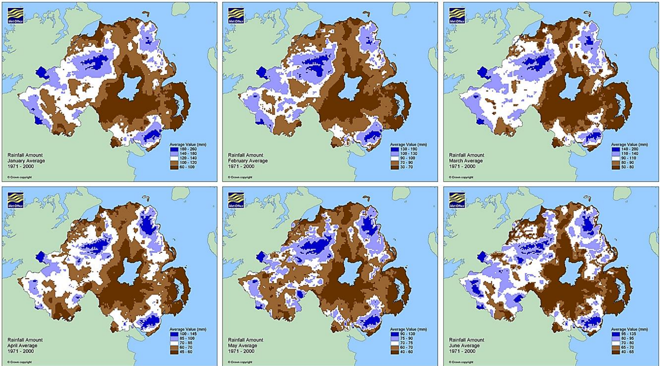
Figure 3.15: Average monthly rainfall (mm) data for January to June from 1971 to 2000 for Northern Ireland (Source: Met Office, 2010).
