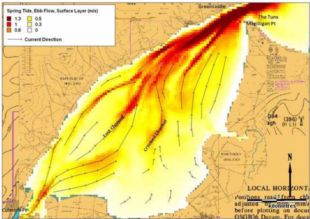
Figure 3.9: Surface current velocities and direction during a spring tide, ebb flow at 21:30:00 November 13 th 2008 (Source: Deltares Delft3D-FLOW).
