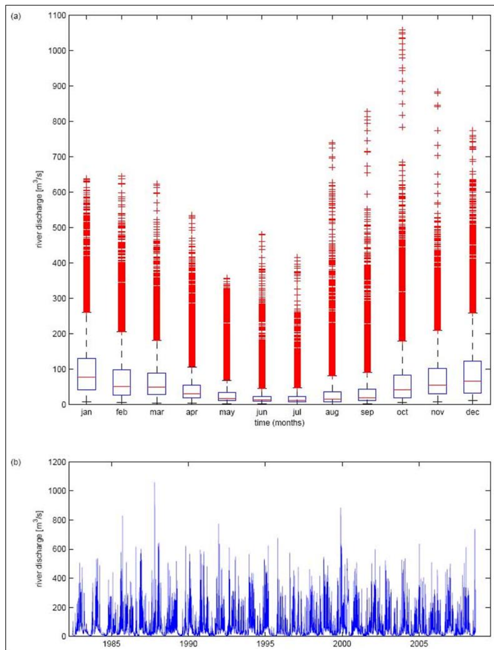
Figure 3.28: River Mourne discharge at Drumnabouy House a) boxplot distribution of discharge per month and b) recorded time series (Source: Deltares, 2009).
