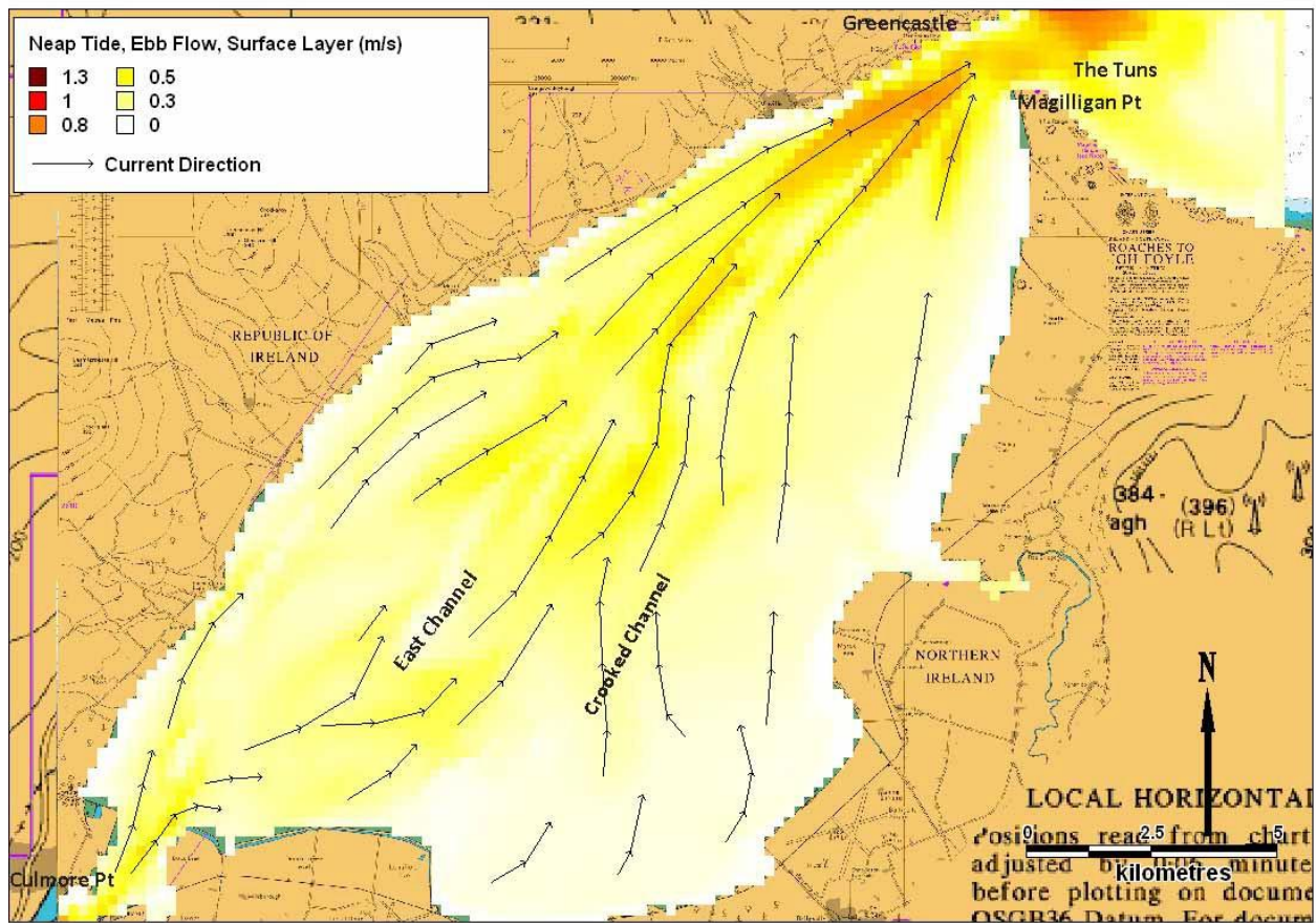
Figure 3.13: Surface current velocities and direction during a neap tide, ebb flow at 15:30:00 November 5 th 2008 (Source: Deltares Delft3D-FLOW).
