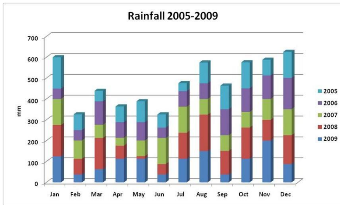
Figure 3.21: Average monthly rainfall (mm) data along the Lough Foyle coast from 2005-2009 (Source: Met Eireann, 2010a).
