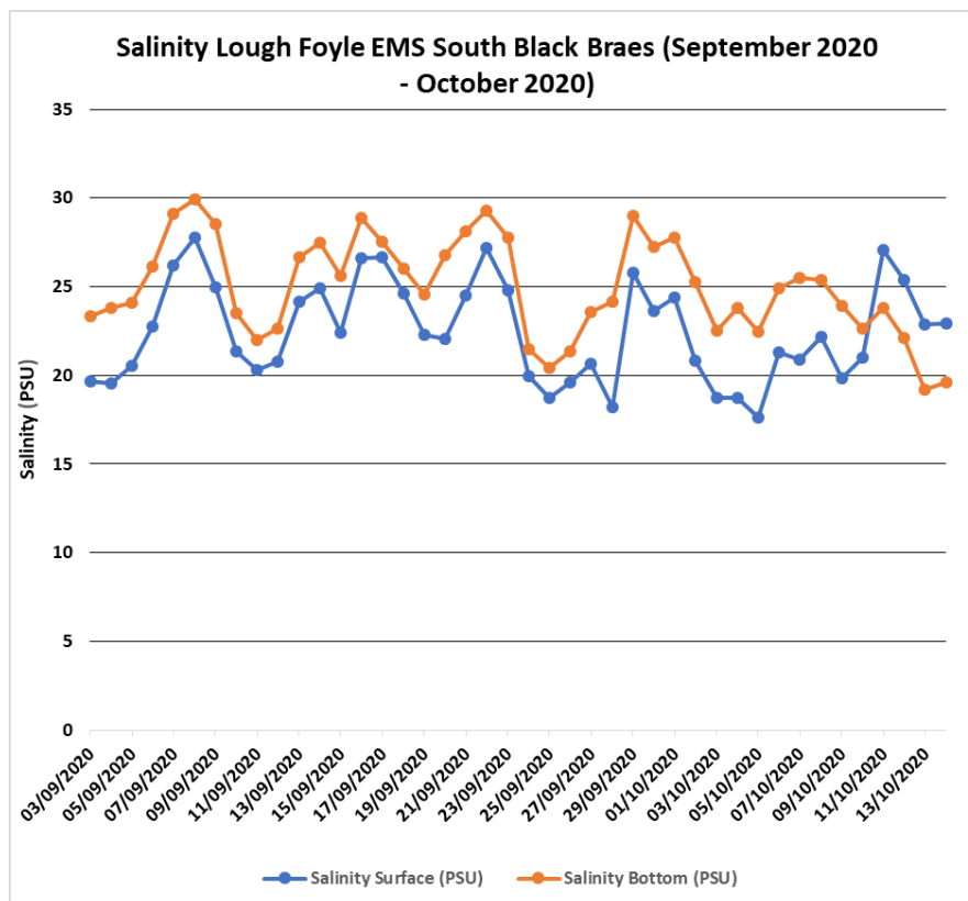
Figure 3.34: Salinity profile at Lough Foyle South EMS from September 2020 to October 2020. (Source: Loughs Agency).
