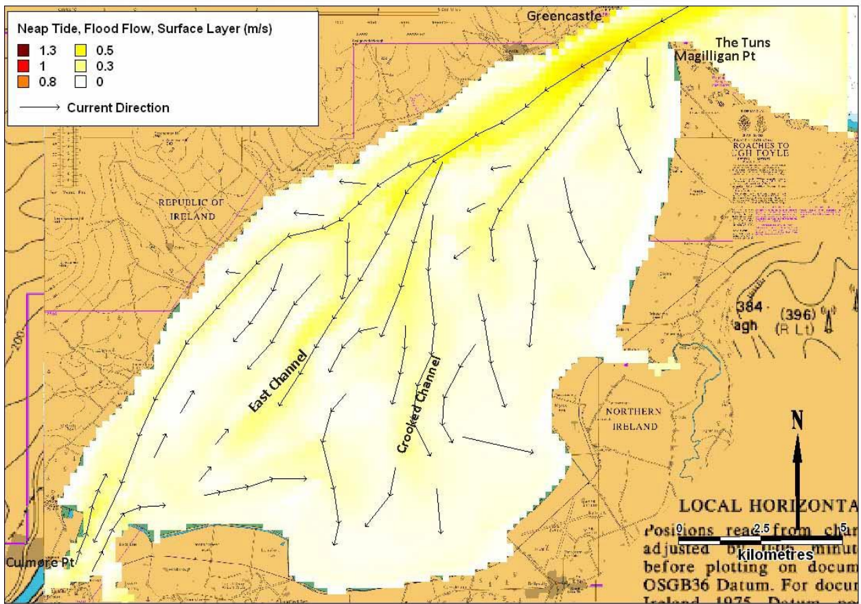
Figure 3.11: Surface current velocities and direction during a neap tide, flood flow at 10:30:00 November 5 th 2008 (Source: Deltares Delft3D-FLOW).
