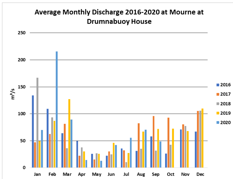
Figure 3.30: Average and monthly flow data from the Mourne at Drumnabuoy House 2016 -2020 (Source: NRFA, 2021)
