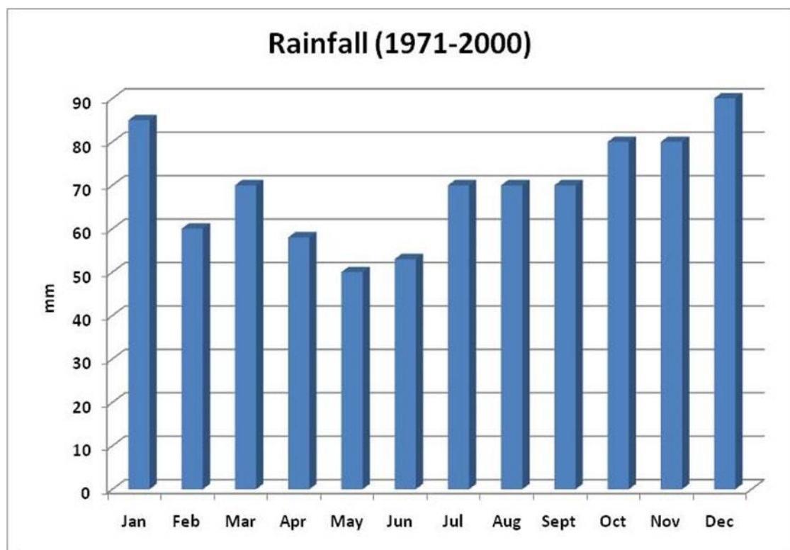
Figure 3.19: Average monthly rainfall (mm) data along the Lough Foyle coast from 1971-2000 (Source: Met Office, 2010).
