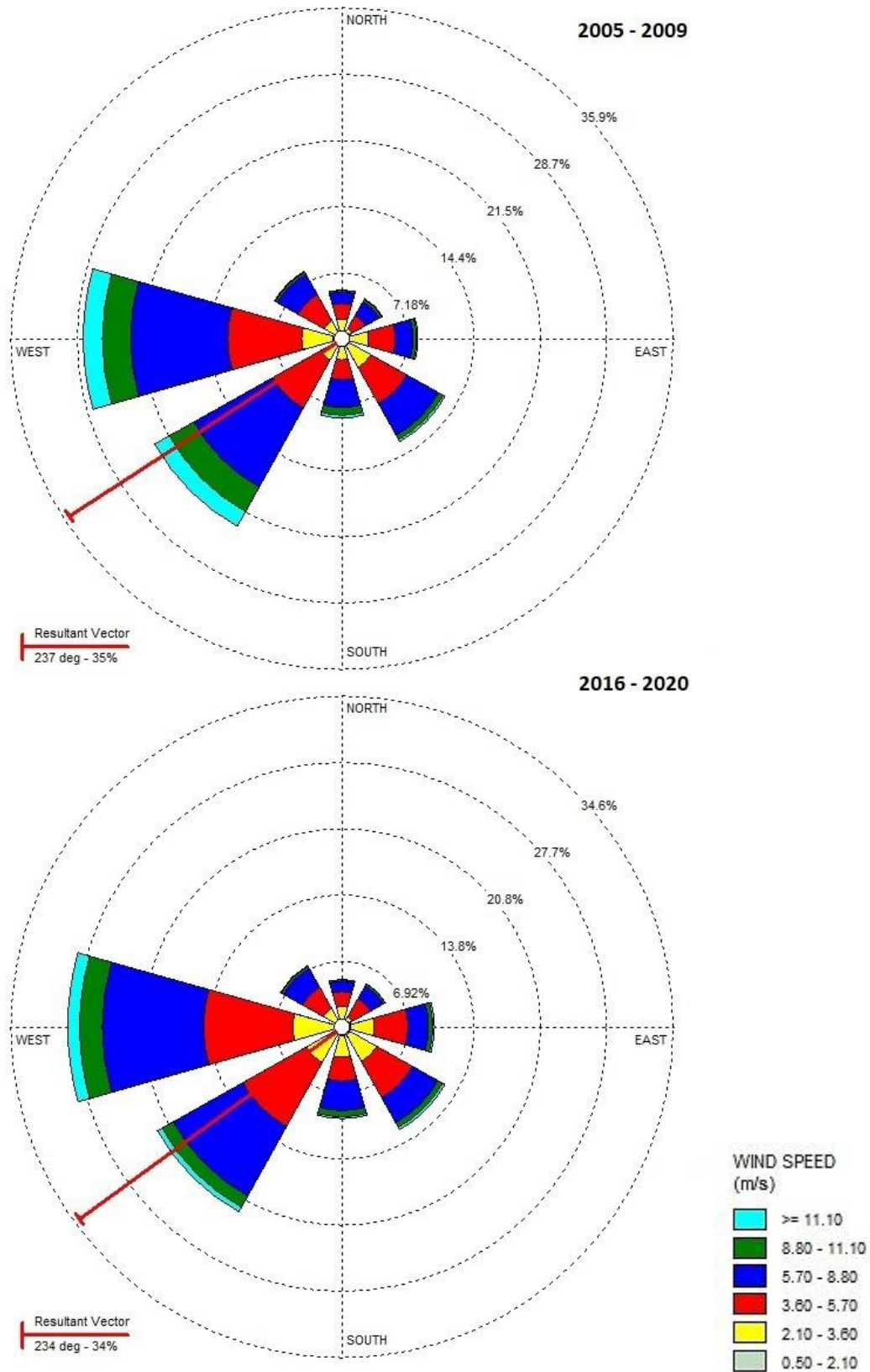
Figure 3.25: Wind roses for Malin Head from 2005 to 2009 and 2015 to 2020. (Source: Met Eireann, 2021a).
