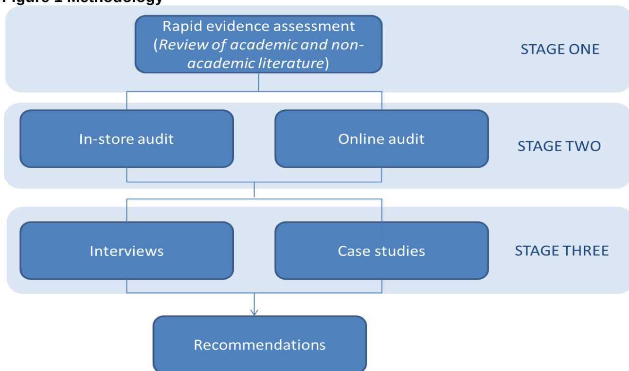
Figure 1 Methodology
